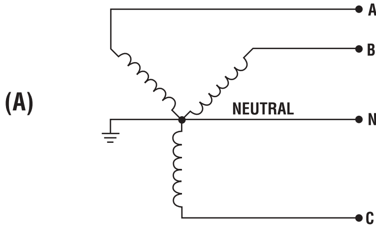
4 Wire Grounded Wye
