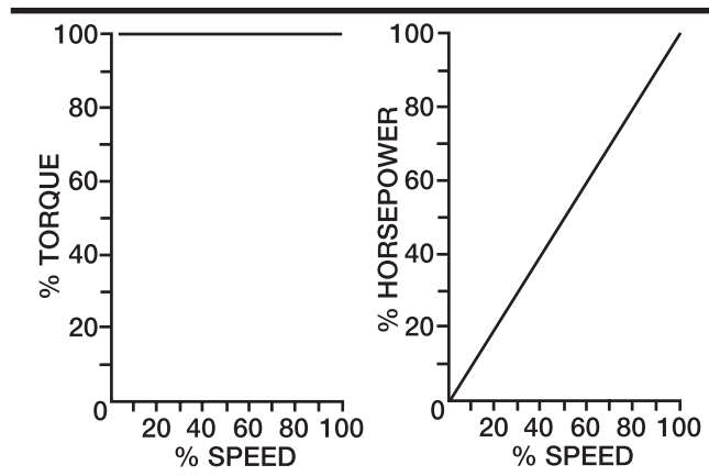
Constant Torque Speed-Torque Relationship
