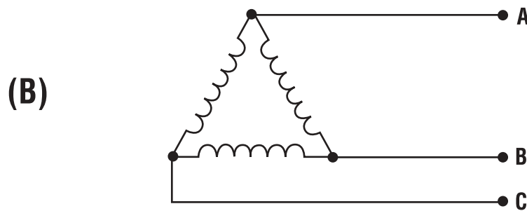
3 Wire Ungrounded Delta
