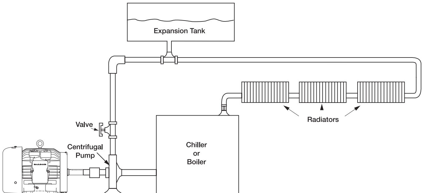
Water Circulation System
