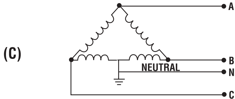
4 Wire Tapped Delta Neutral Grounded
